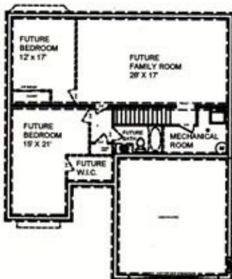
BASEMENT PLAN SCALE: 1/8" = 1'-0"
