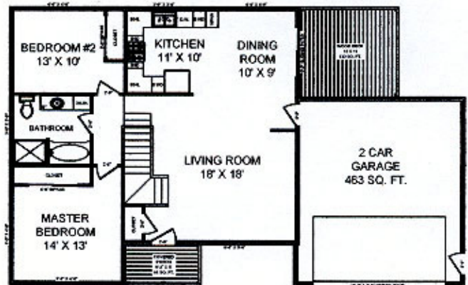
MAIN FLOOR PLAN SCALE: 1/8" = 1'-0" NTS
